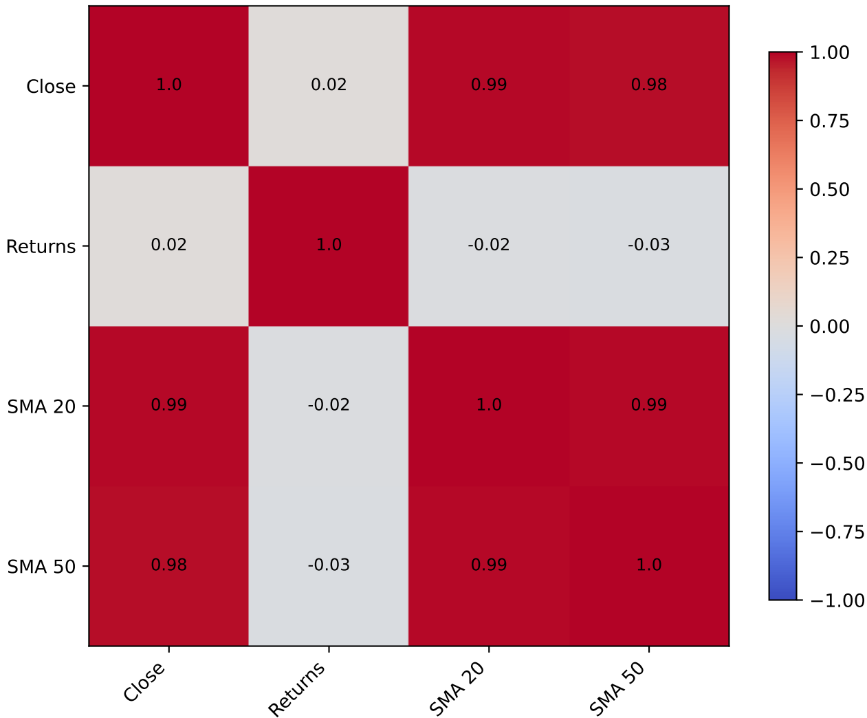
Correlation matrix
